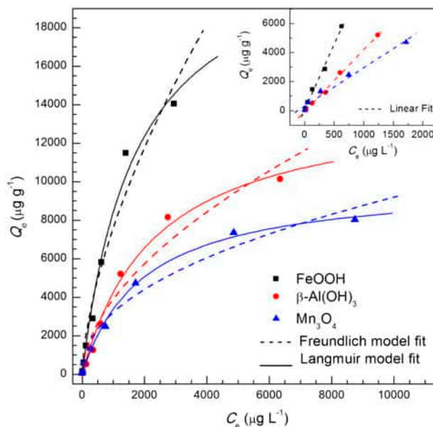
Fig. 4. Adsorption isotherms of As(V) by ferrihydrite (FeOOH), bayerite ( \beta -Al(OH) 3 ), and hausmannite (Mn 3 O 4 ) in 0.1 M NaCl at 298 \pm 1 \text{ K} . Inset is As(V) adsorption isotherms in the C_e ( \text{mg L}^{-1} ) range of 0–2.00 and their linear fits.
