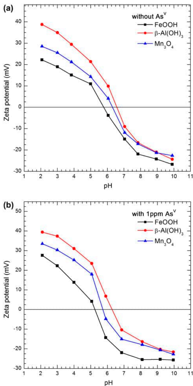
Fig. 2. Zeta potential ( \zeta ) profiles of ferrihydrite ( \text{FeOOH} ), bayerite ( \beta\text{-Al}(\text{OH})_3 ), and hausmannite ( \text{Mn}_3\text{O}_4 ) vs. pH in 0.1 \text{ M NaCl} solution (a) without \text{As}(\text{V}) and (b) with 1 \text{ ppm} ( 4.25 \text{ }\mu\text{M} ) \text{As}(\text{V}) at 298 \pm 1 \text{ K} .
