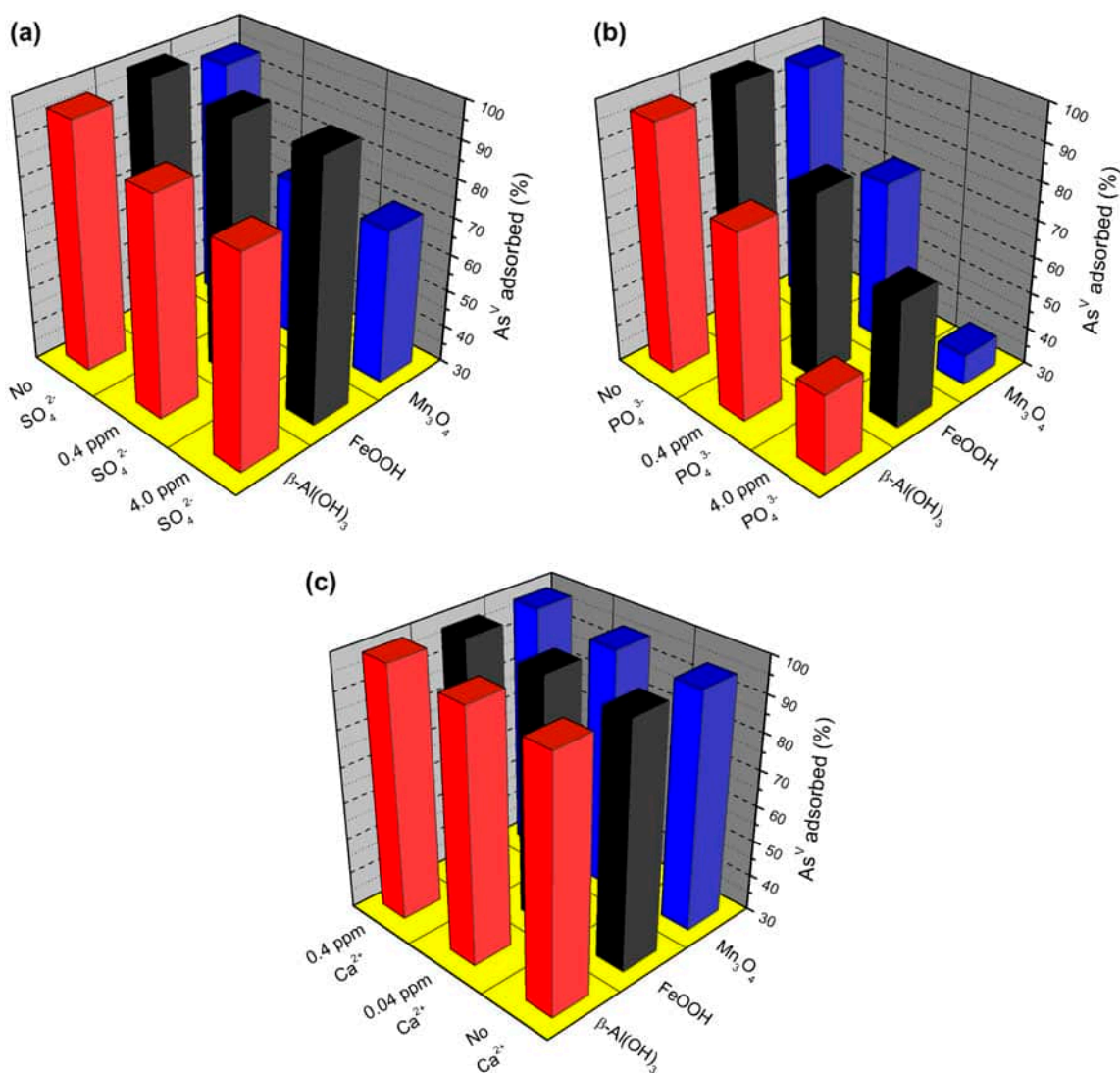
Fig. 6. Effect of \text{SO}_4^{2-} (a), \text{PO}_4^{3-} (b), and \text{Ca}^{2+} (c) on As(V) adsorption in 0.1 M NaCl at 298 ± 1 K.
