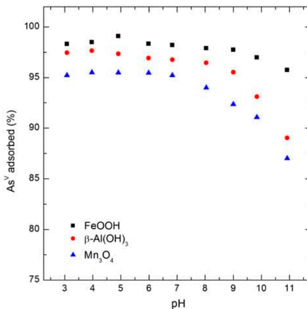
Fig. 3. Uptake envelopes of As(V) by ferrihydrite (FeOOH), bayerite ( \beta -Al(OH) 3 ), and hausmannite (Mn 3 O 4 ) in 0.1 M NaCl solution upon 24 h reaction at 298 \pm 1 \text{ K} (initial As(V): 0.4 \text{ mg L}^{-1} , eq. 1.28 \mu\text{M} ).
