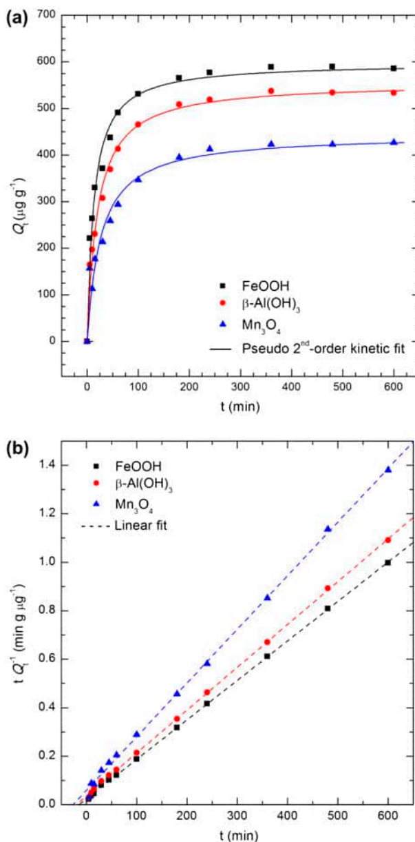
Fig. 5. Kinetic curves of As(V) adsorption by ferrihydrite (FeOOH), bayerite ( \beta\text{-Al(OH)}_3 ), and hausmannite ( \text{Mn}_3\text{O}_4 ) in 0.1 M NaCl at 298 \pm 1 \text{ K} . (a) Q_t \sim t ; (b) t Q_t^{-1} \sim t (initial [\text{As(V)}]: 0.67 \text{ mg L}^{-1} , eq. 8.84 \mu\text{M} ). All initial pH values were adjusted to 6.0 \pm 0.1 with dilute HCl and NaOH.
