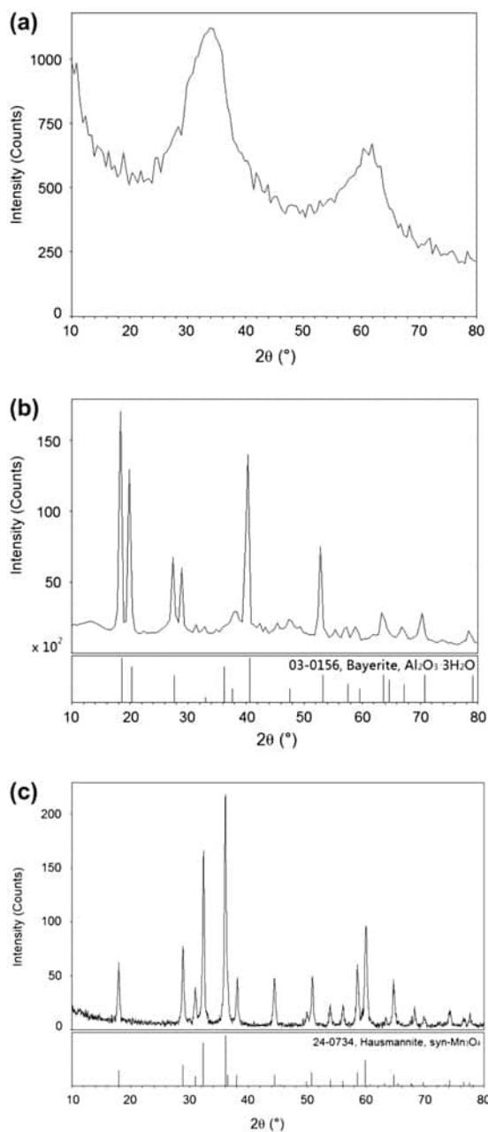
Fig. 1. XRD patterns of synthetic (a) ferrihydrite, (b) bayerite, and (c) hausmannite.
