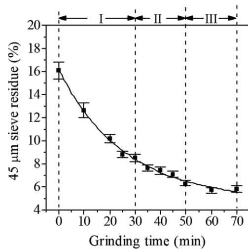
Fig. 2. Variation of 45 μm sieve residue of CFBC fly ash with grinding time (square mesh sieve).
